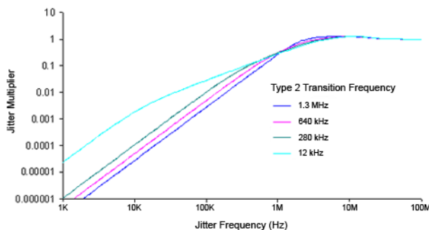
Figure 9-1. OJTF for 5 MHz LBW vs. Type-2 Transition Frequency
