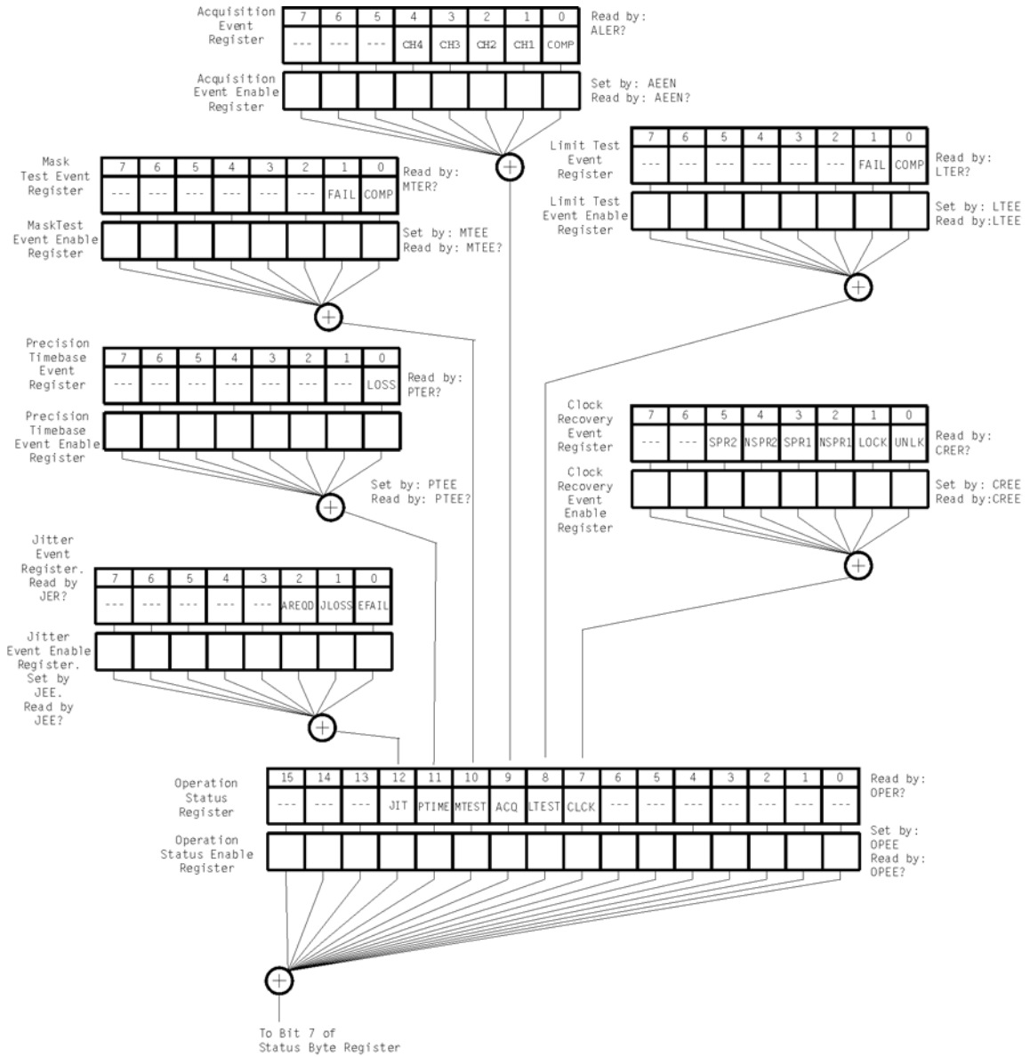
Figure 1-8. Status Reporting Data Structures
